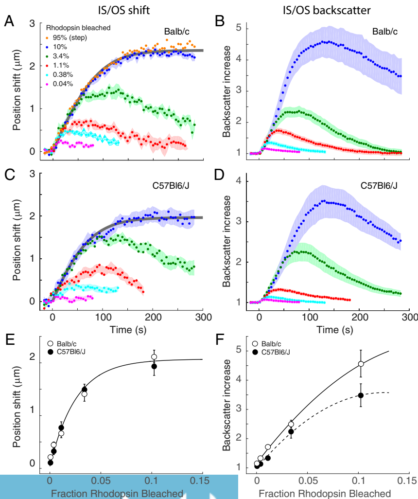
Fig. 3. Rhodopsin bleach dependence and kinetics of rod elongation and backscattering increases. Results were obtained with the experimental paradigm of Fig. 1, using both albino (BALB/c) mice (A and B) and pigmented (C57Bl6/J) mice (C and D) with light exposures that bleached between 0.04% and 95% of the rhodopsin (symbol key in A). E and F plot the dependence of the amplitudes of the elongation (E) and IS/OS backscatter increases as a function of the bleach level. The smooth curve in E is an exponential function that reaches 1- e^{-1} of the saturated level at a 2.6% level of bleaching; the smooth curves in F are quadratic functions that serve to highlight the declining rate of backscatter increase with increasing bleach level. In A–D the symbols plot mean values, and the colored backgrounds plot the SEMs of the traces. Each trace is the average of at least 6 experiments from both eyes of at least three mice. For the lower bleach levels up to 44 individual experiments were averaged. (OCT data collection was truncated short of 300 s in the experiments with the three lowest bleach levels.) The fraction bleached can be converted into photoisomerizations per rod ( R^* ) by multiplying by 7 \times 10^7 , the average number of rhodopsin molecules per mouse rod (81).
